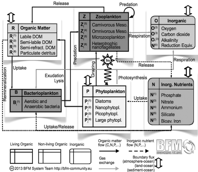
Fig. 1. The standard BFM configuration
