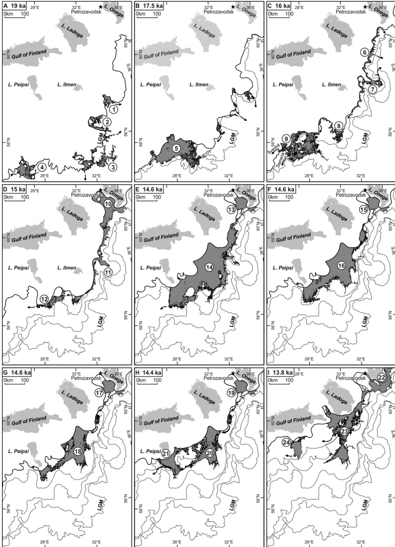
Fig. 2. Time slice reconstruction of large (>1000 km 2 ) proglacial lakes at southeastern flank of Scandinavian Ice Sheet 19–13.8 ka BP. Numbers indicate the lake in Table; lake characteristics shown in Table; arrows indicate the drainage direction
